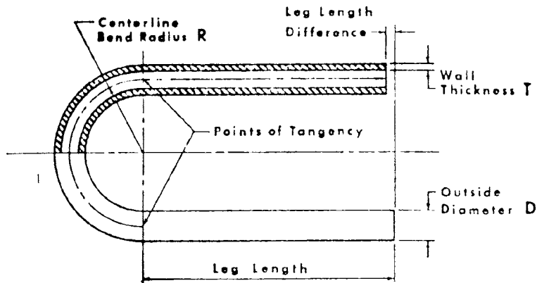
FIG. S1 Bent Portion of U-Tube
